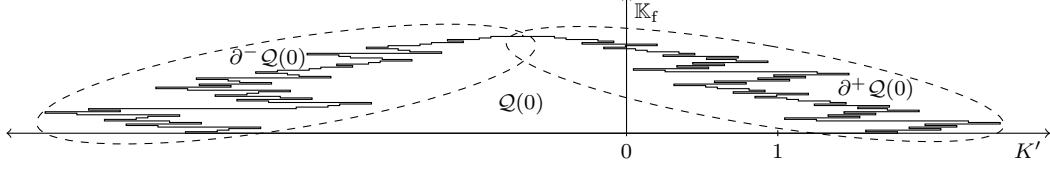
Figure 1: The two boundaries of the tile \mathcal{Q}(0) for \beta = 1 + \sqrt{3} .
